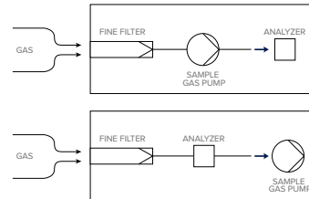
PRINCIPLE OF GAS SAMPLING GAS DETECTION PORTABLE
